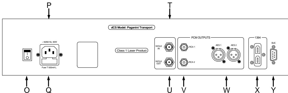
Figure 6 - Rear Panel
